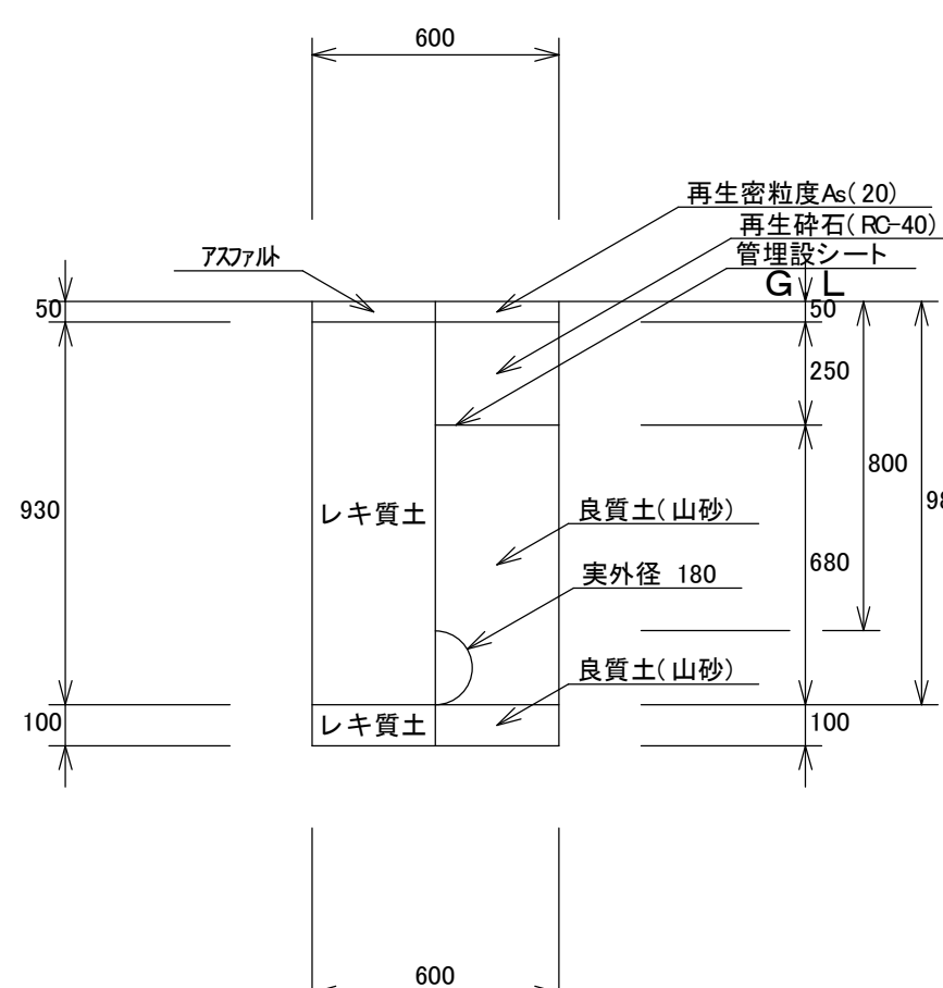
00: 配水管 12: \Phi 150 H=0.8m (A 2 ) (掘削: 掘削) 1/2
